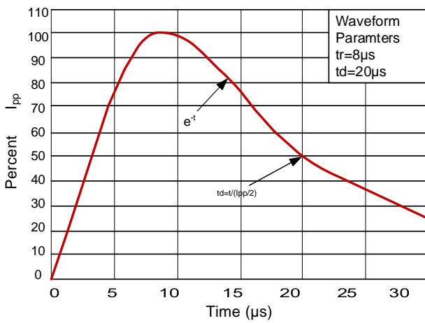
Figure3: Pulse Waveform
