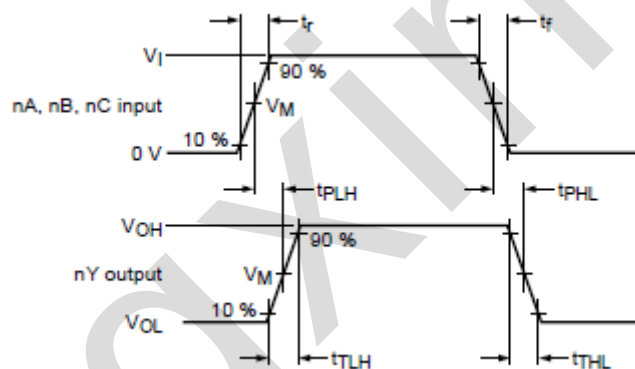
Figure 4. Input to output propagation delay and output transition times
