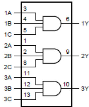
Figure 1. Functional diagram
