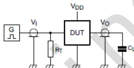
Figure 4. Test circuit for switching times
