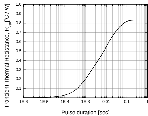
Figure 6. Thermal Resistance
