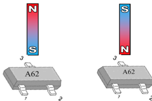
V OUT =低电压 V OUT =高电压 SOT23 (AH602)
