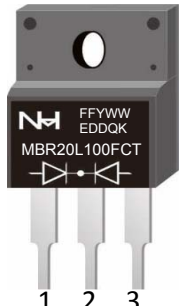
TO-220F MBR20L100FCT
