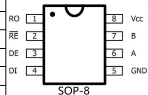
SOP-8
