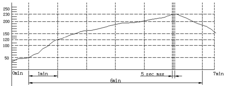
Time inside soldering equipment Temperature Profile
