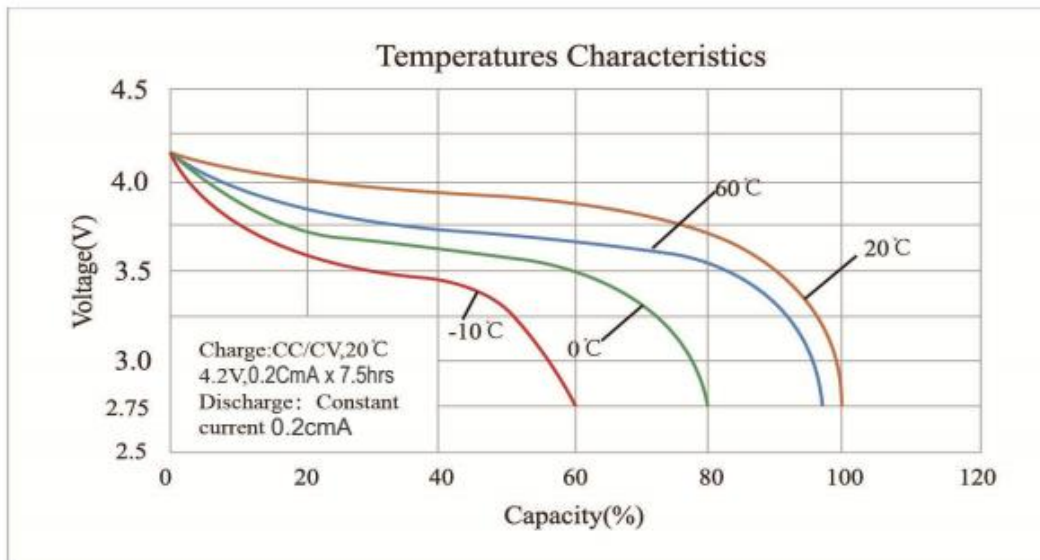
Fig. 3 Discharging Characteristics at various Temperatures
