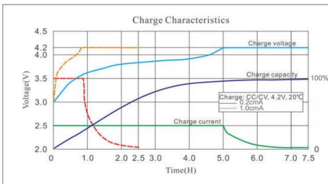
Fig.1 Charging Characteristics at various currents
