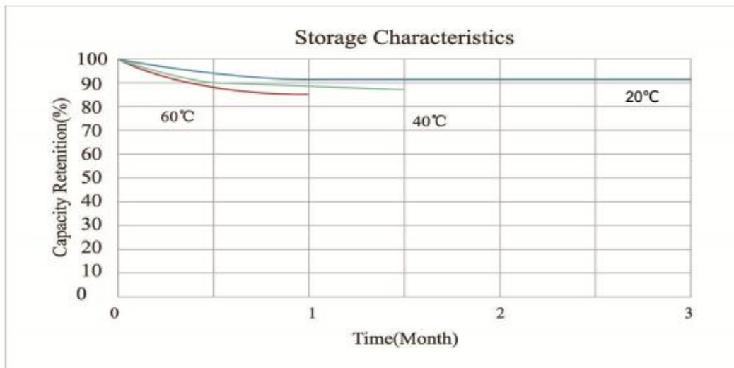
Fig. 4 Storage Characteristics
