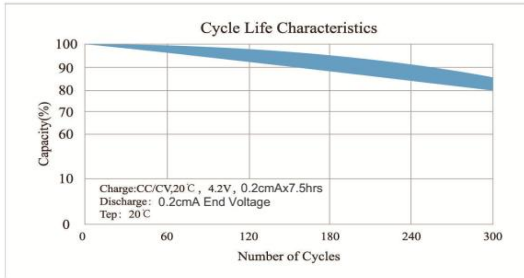
Fig. 5 Cycle Life Chart
