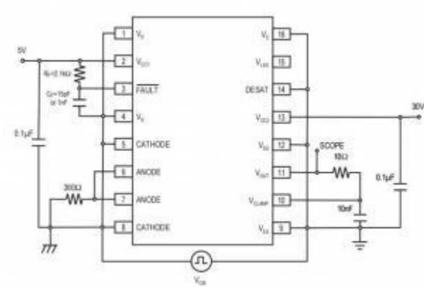
Figure 33. CMR Test Circuit LED1 On
