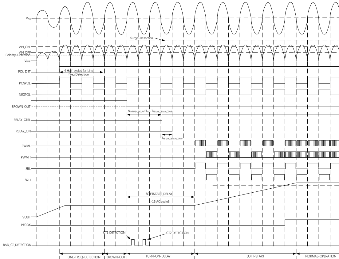
Figure 31 Start-up Sequence
