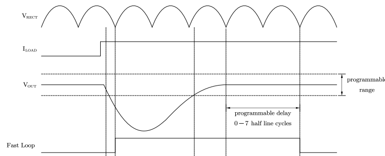
Figure 29 Fast Loop for Transient Response Improvement
