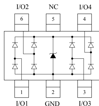
SOT23-6L (Top View)
