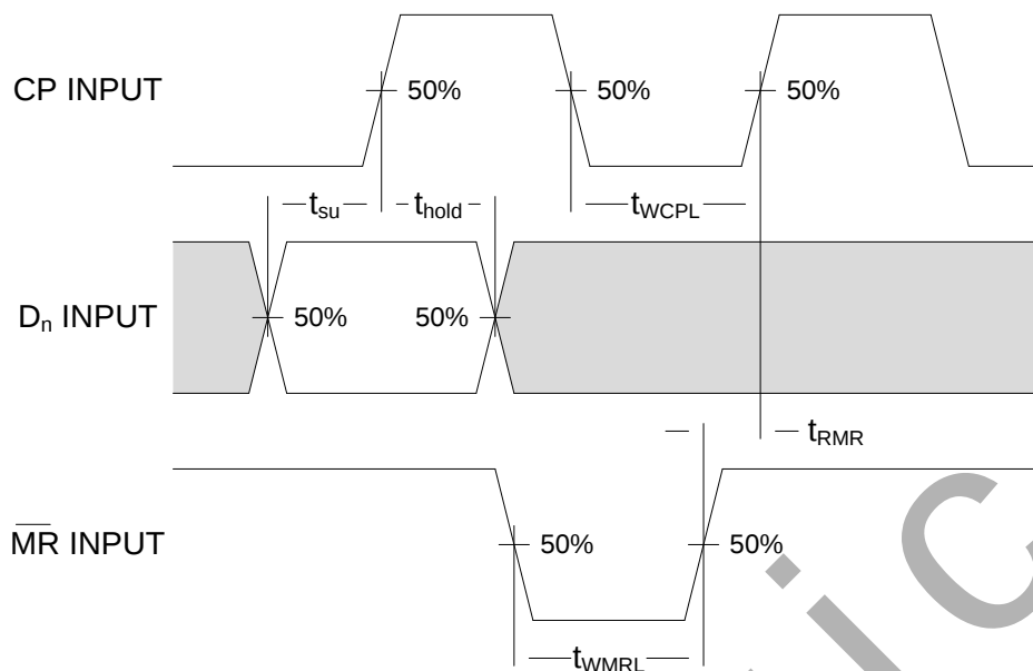
Figure 5. Waveforms showing minimum pulse widths for CP and MR, MR to CP recovery time, and set-up time and hold time for D n to CP. Set-up and hold times are shown as positive values but may be specified as negative values.
