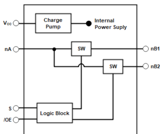
Figure 2 Functional Block Diagram
