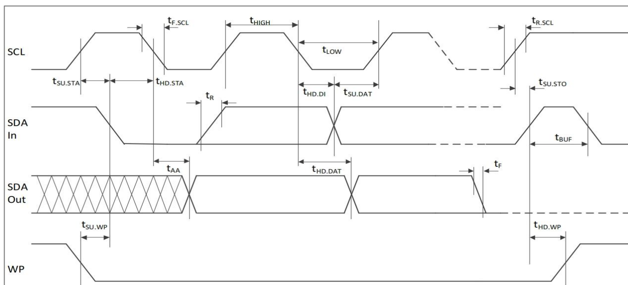
Figure 6-1 Bus Timing
