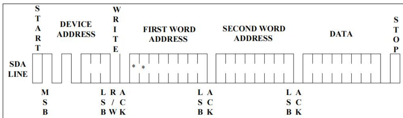
Figure 5. Byte Write
