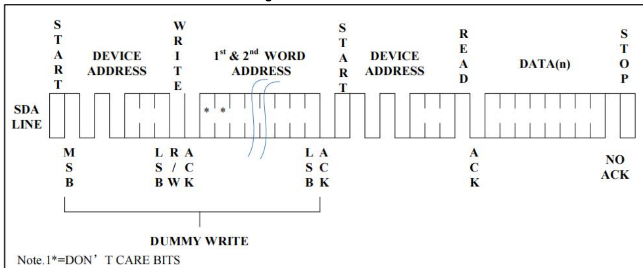
Figure 9. Sequential Read
