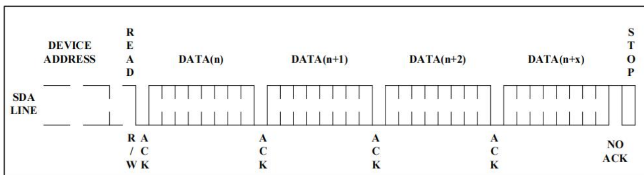
Figure 9. Sequential Read
