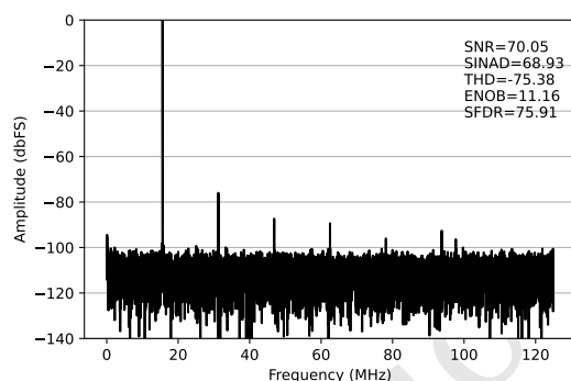
(b) 输入信号频率 = 28MHz
