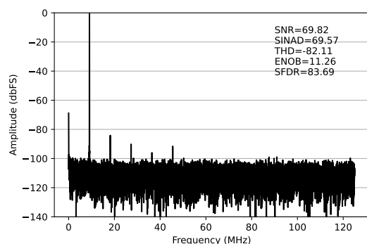
(a) 输入信号频率 = 10MHz
