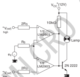
LIMIT COMPARATOR
