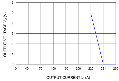
Fig.8 Current Cut-off Grid Voltage
