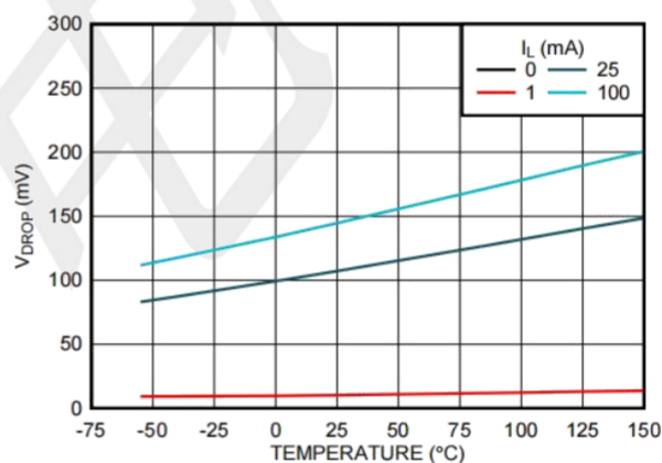
Dropout Voltage ( V_{DRO} ) versus Temperature
