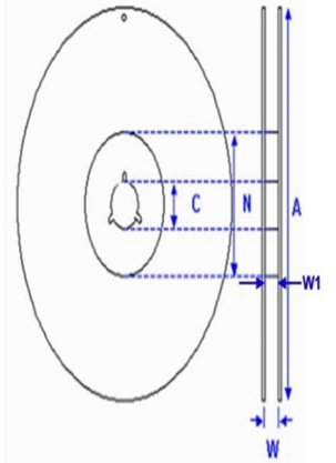
Fig. 9.1 The dimension of reel
