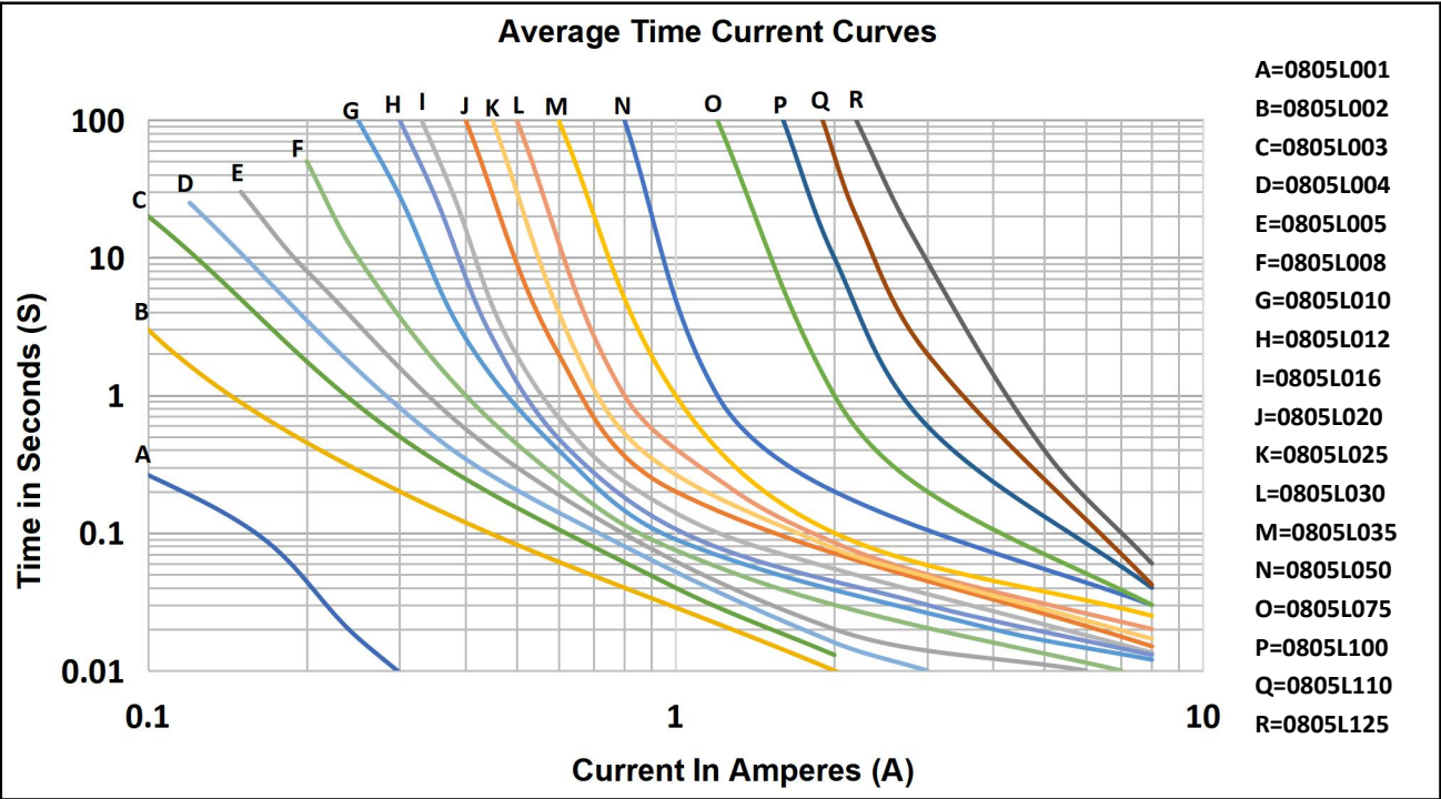
Typical Time-to-Trip at 25°C/25°C跳闸保护时间曲线表
