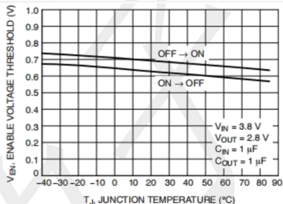
Figure 2 Enable Thresholds Voltage
