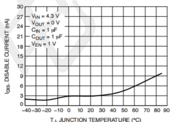
Figure 4 Disable Current vs. Temperature
