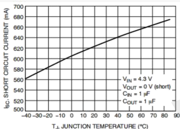
Figure 1 Short Circuit Current vs. Temperature
