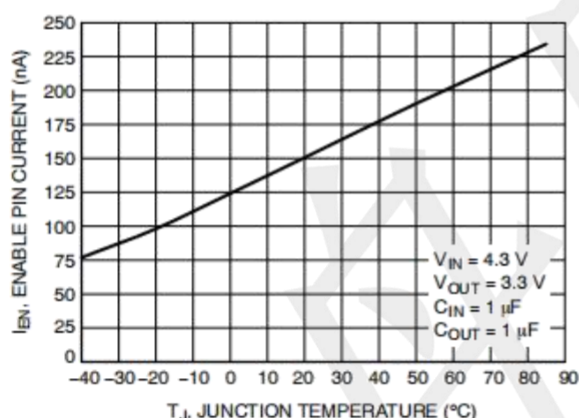
Figure 3 Current to Enable Pin vs. Temperature
