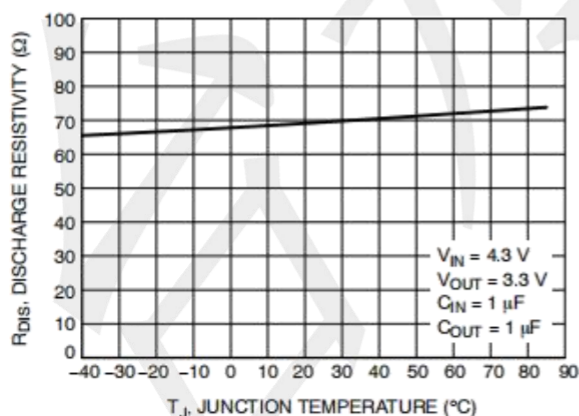
Figure 5 Discharge Resistance vs. Temperature
