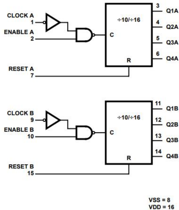
Figure 2.2 Functional Diagram
