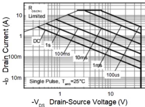
P-channel Safe Operating Area
