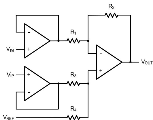
Figure 6. Instrument Amplifier
