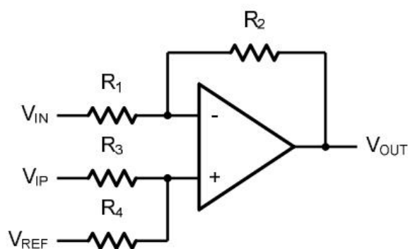
Figure 4. Differential Amplifier
