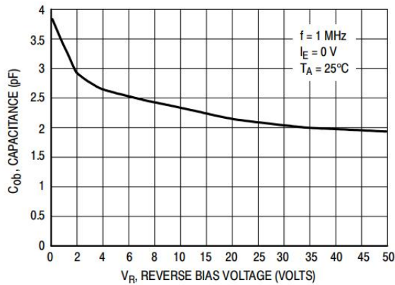
Figure 03. Output Capacitance
