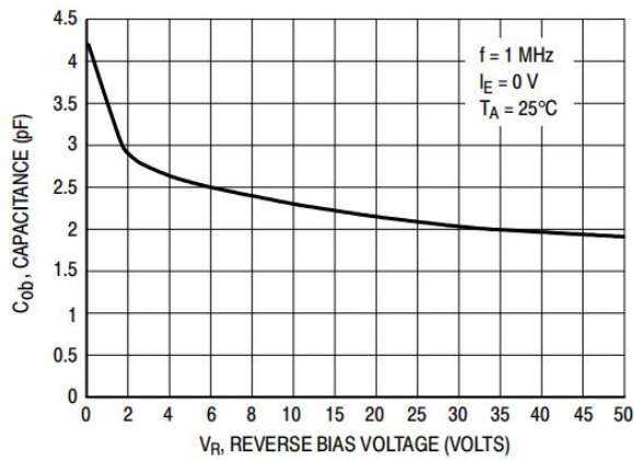
Figure 03. Output Capacitance
