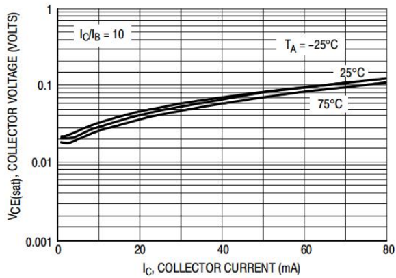
Figure 01. V_{CE(sat)} versus I_C
