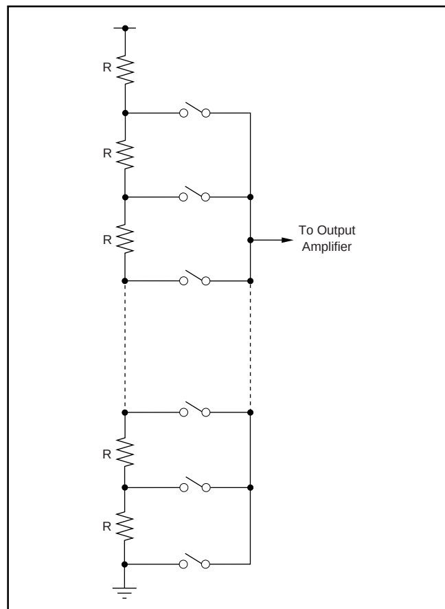
FIGURE 2. Resistor String.
