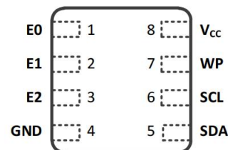
DFN-8 2*3
