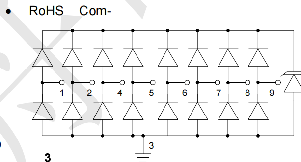
Circuit Diagram
