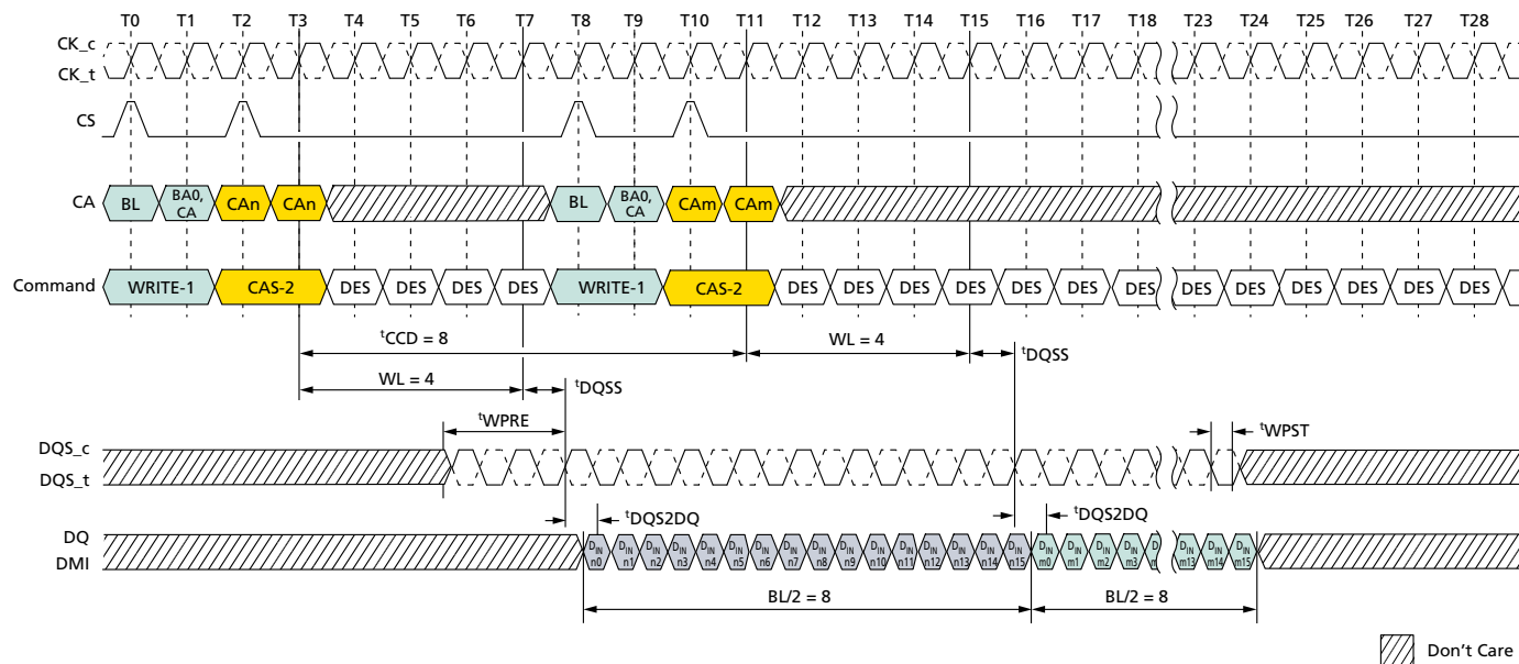
Figure 52: Seamless WRITE: t_{\text{CCD}} = \text{MIN} , 0.5n\text{CK} Postamble
