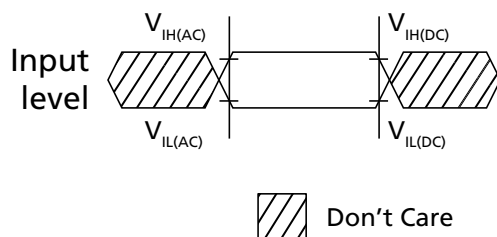
Figure 147: Input Timing Definition for CKE
