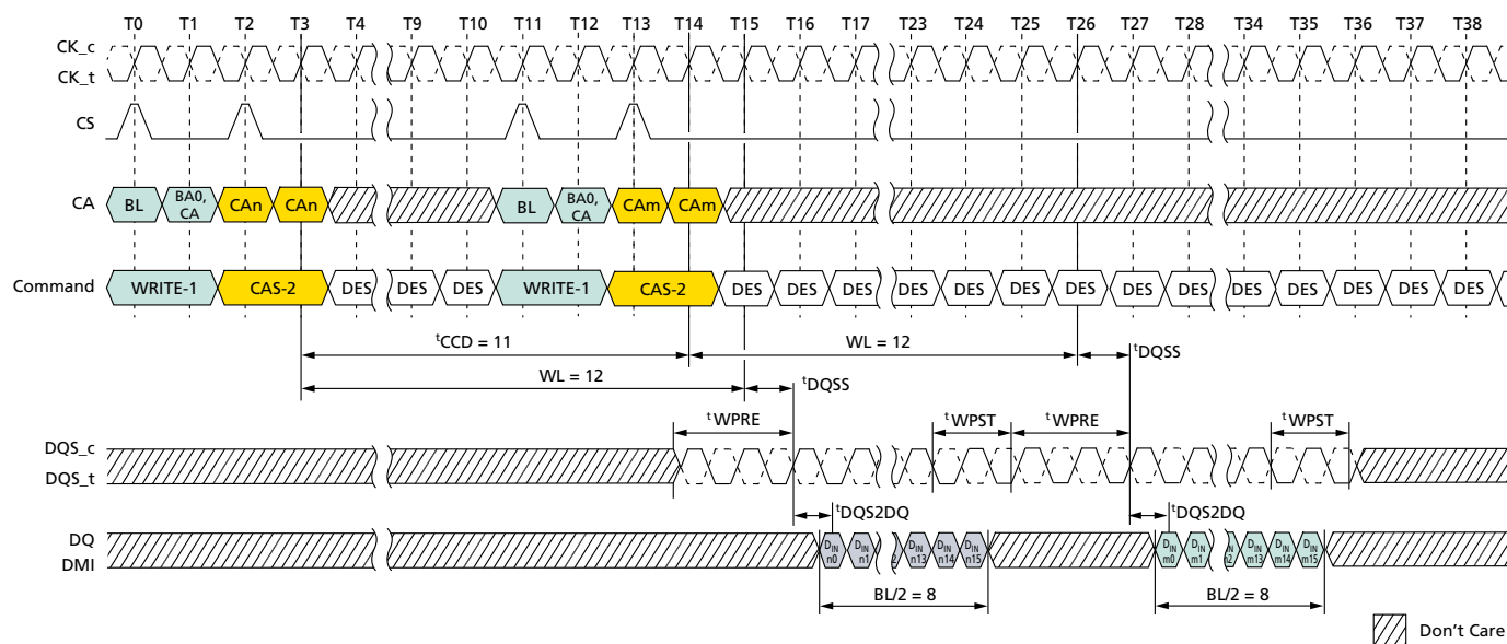
Figure 60: Consecutive WRITE: t_{CCD} = MIN + 3, 1.5nCK Postamble
