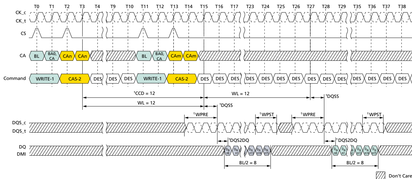
Figure 61: Consecutive WRITE: t_{CCD} = MIN + 4, 1.5nCK Postamble
