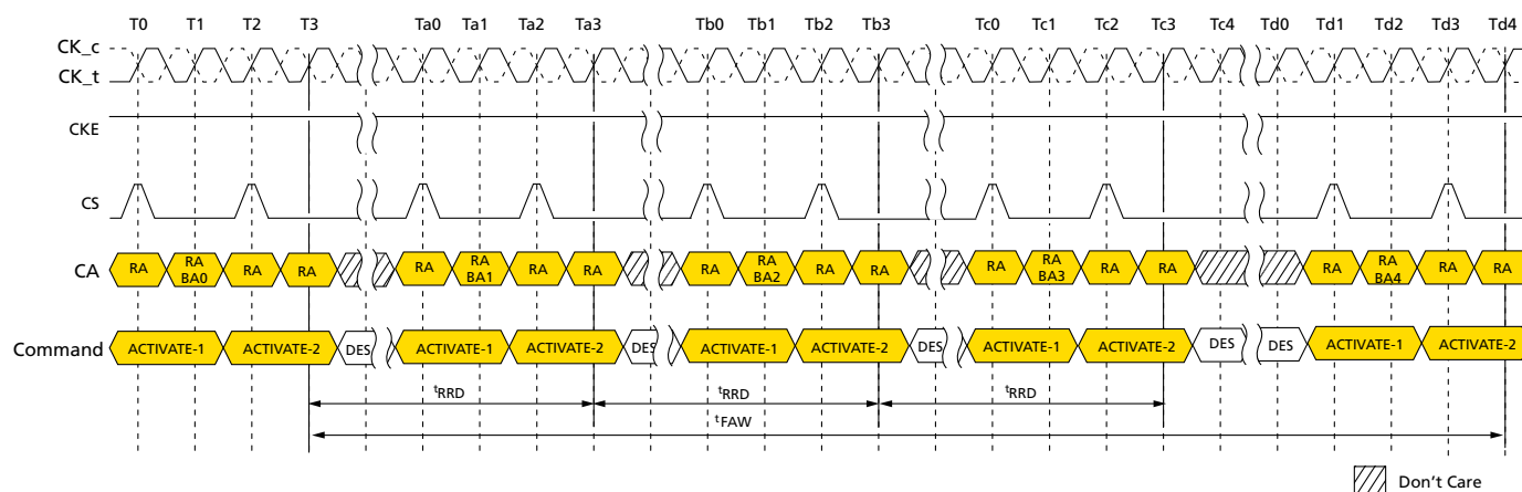
Figure 13: t_{FAW} Timing
