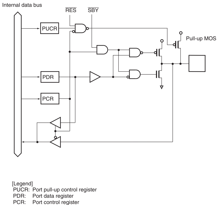
Figure B.4 Port 1 Block Diagram (P11)
