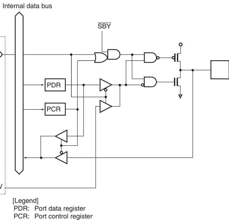
Figure B.11 Port 7 Block Diagram (P76)
