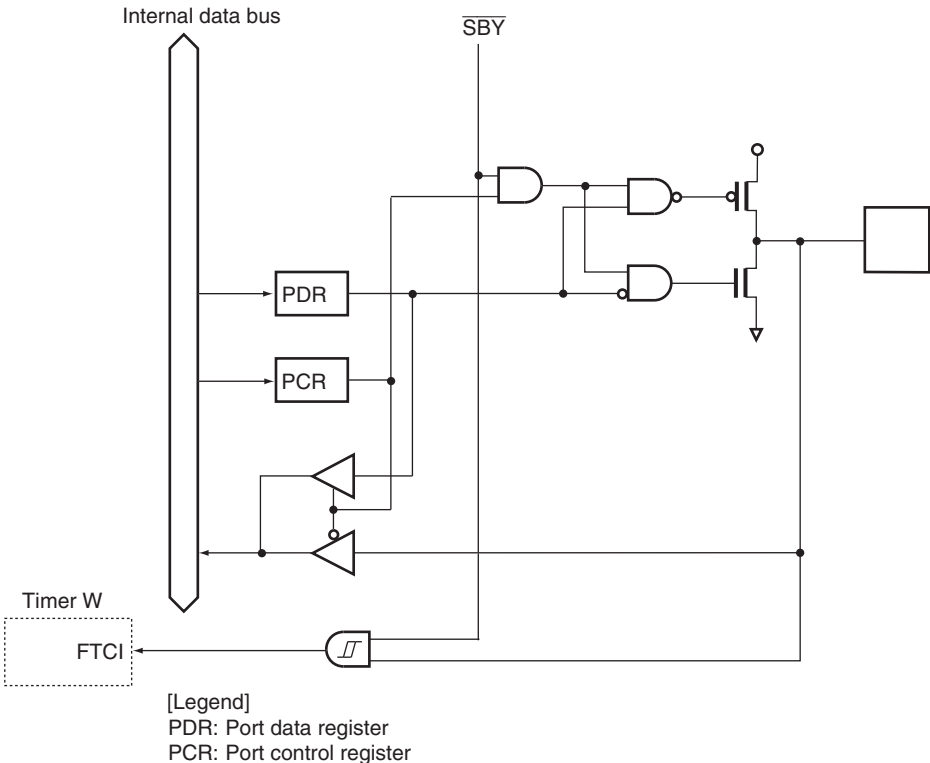
Figure B.15 Port 8 Block Diagram (P80)
