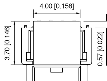
PICK AND PLACE AREA WITH CAP
