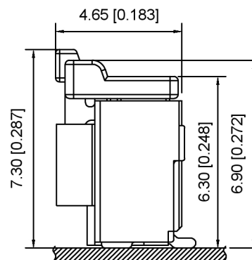
PICK AND PLACE AREA WITH CAP
