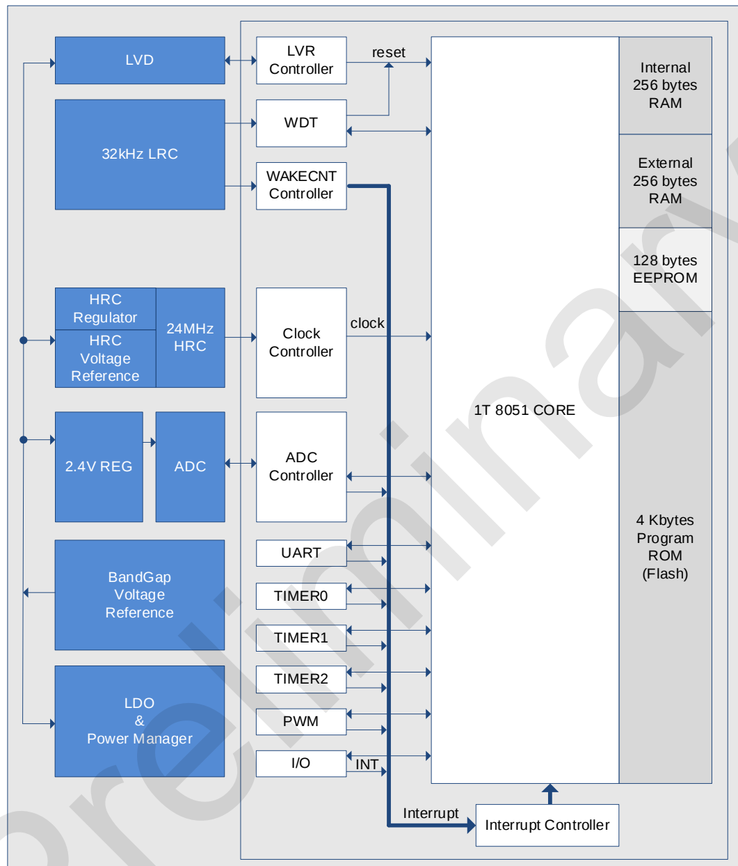
SC92F720X BLOCK DIAGRAM
