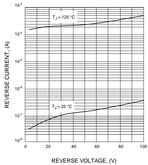
FIG.4 - TYPICAL REVERSE CURRENT
