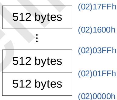
SC95F861XB EEPROM Sector 分区示意
