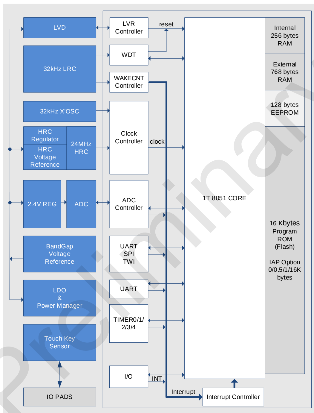
SC92F84HX BLOCK DIAGRAM
