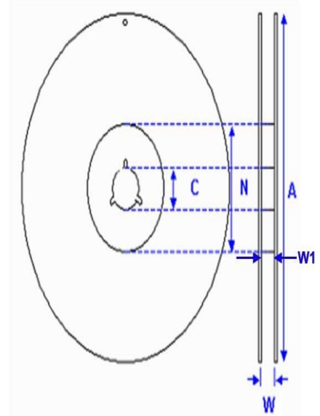
Fig. 9.3 The dimension of reel
