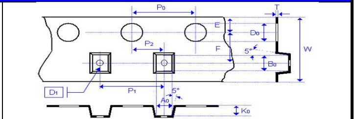
Fig. 9.2 The dimension of plastic tape
