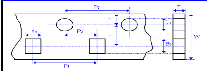
Fig. 9.1 The dimension of paper tape
