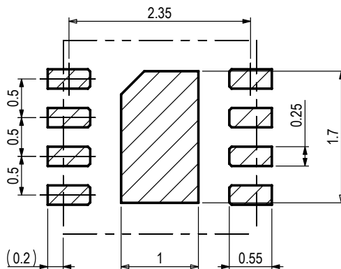
Figure 8 Recommended metal land pattern (left) and stencil apertures (right) for the STS3xA-DIS. The dashed lines represent the outer dimension of the DFN package. The PCB pads (left) and stencil apertures (right) are indicated through the shaded areas.
