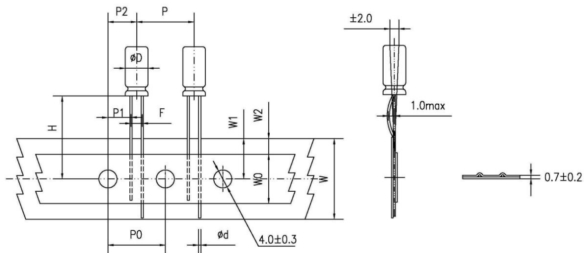
DIMENSIONS(mm)
