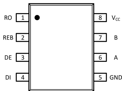
(c) SOIC8
