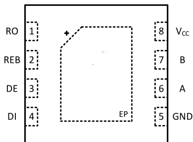
(a) DFN8
