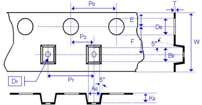
Fig. 9.2 The dimension of plastic tape
