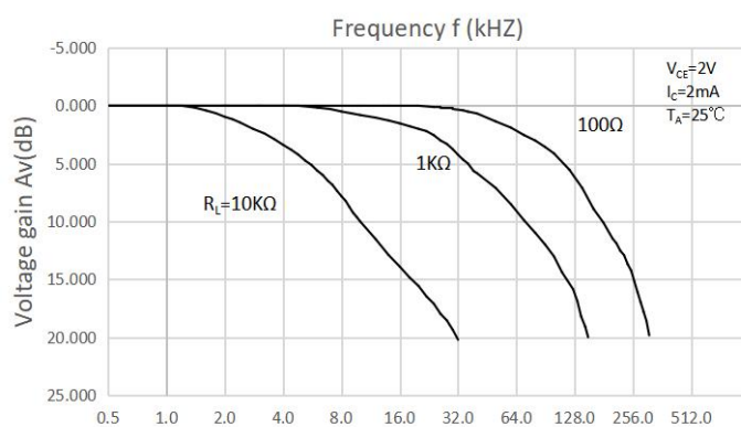
Fig.11 Frequency Response
