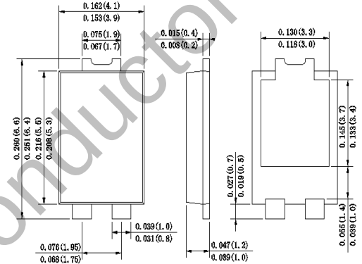
TO-277B
