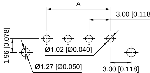
PCB LAYOUT
