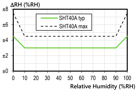
Figure 2. SHT40A typical and aximal relative humidity accuracy at 25 °C.
