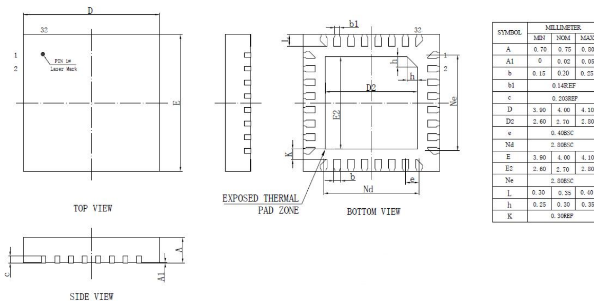
Figure 3-1 JL6976M Package
