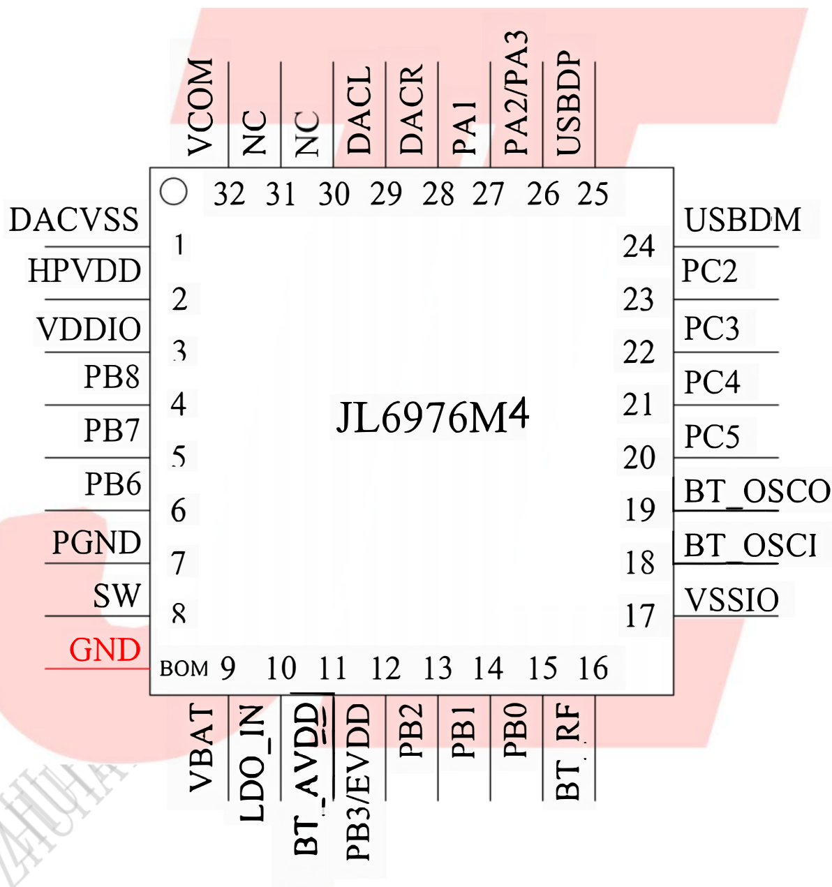
Figure 1-1 JL6976M Package Diagram
