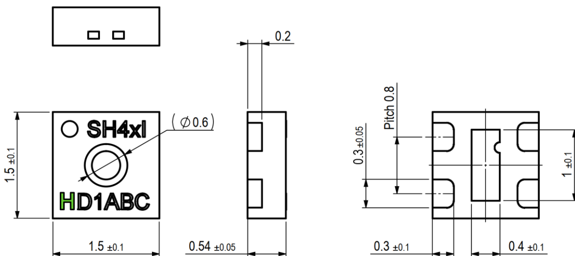
Figure 4. Dimensional drawing of SHT4xl-Analog including package tolerances (units mm), where the H (here highlighted in green for better identification) serves as indicator for the standard analog interface. Other letters alphabetically after the letter H, indicate other versions of the analog interface.
