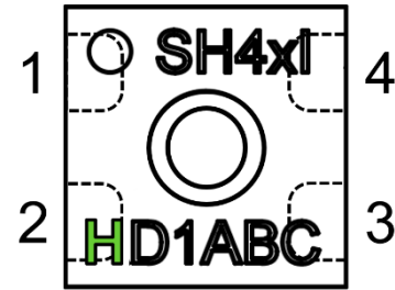
Figure 7. Pin assignment (transparent top view). Dashed lines are only visible if the sensor is viewed from below. The die pad is not directly connected to any pin.
