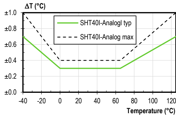
Figure 2. SHT40I analog typical and maximal temperature accuracy.
