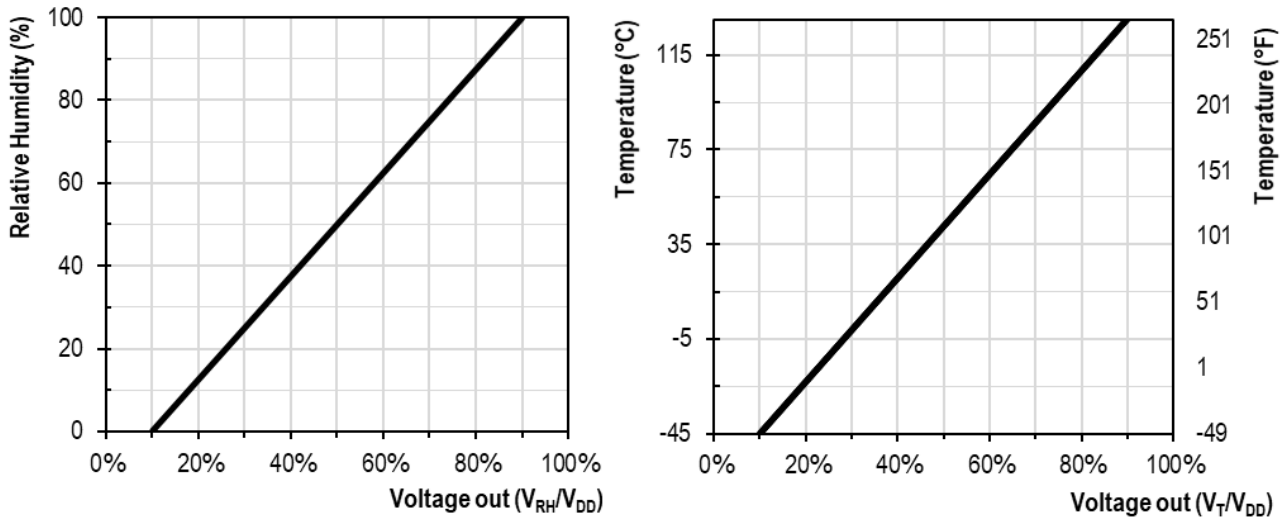
Figure 3. Relationship between the analog voltage output and the measured relative humidity and temperature corresponding to equations ( 1 ) ( 2 ) & ( 3 )for the SHT40I-HD1B.
