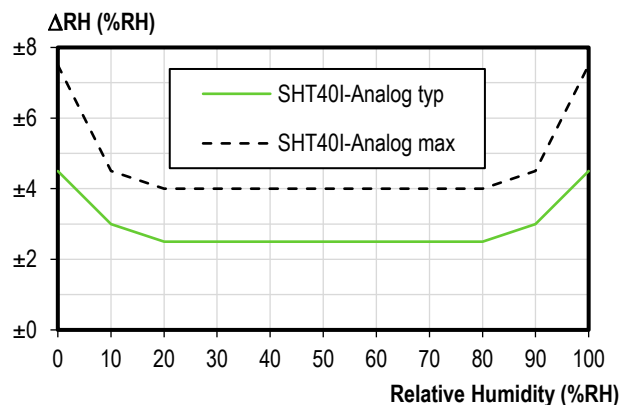
Figure 1. SHT40I-Analog typical and maximal relative humidity accuracy at 25 °C.
