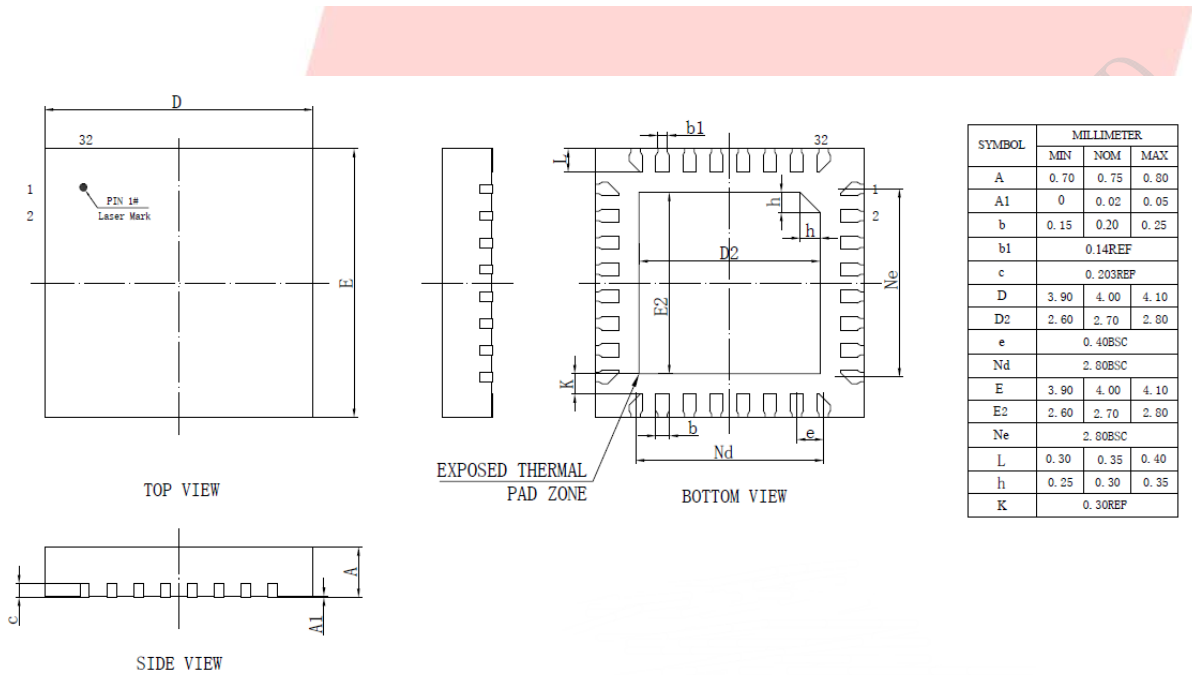
Figure 3-1 AC7006D Package
